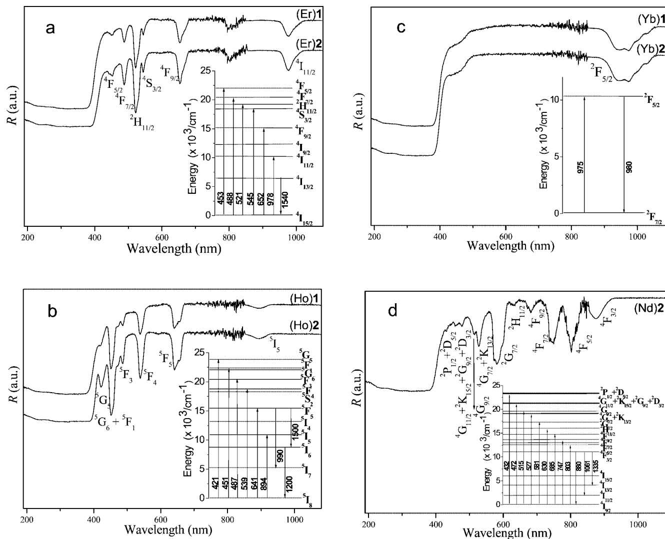
Figure 4. DR spectra of (Er)1 and (Er)2 (a), (Ho)1 and (Ho)2 (b), (Yb)1 and (Yb)2 (c), and (Nd)2 (d). The insets show the energy level diagrams of \text{Er}^{3+} , \text{Ho}^{3+} , \text{Yb}^{3+} , and \text{Nd}^{3+} . The transitions of the bands [nm] are indicated by arrows.
