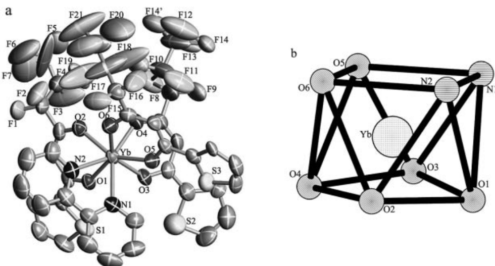
Figure 2. ORTEP plot for (Yb) 2 with ellipsoids drawn at the 30% probability level. Hydrogen atoms have been omitted for clarity.
