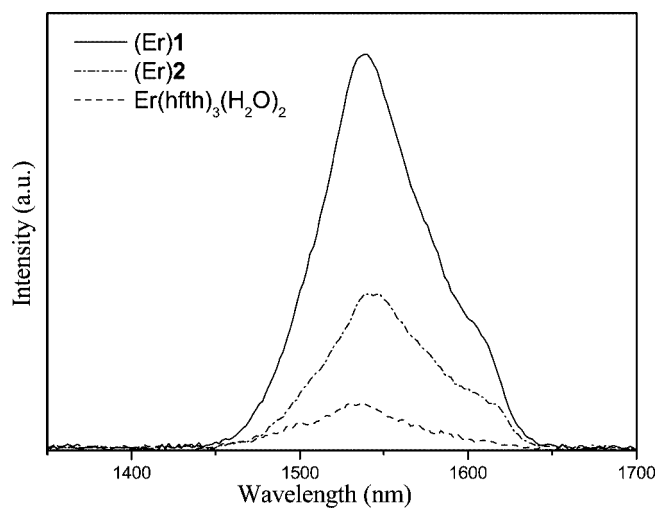
Figure 5. Emission spectra ( \lambda_{\text{ex}} = 397 \text{ nm} ) of (Er)1, (Er)2, and [\text{Er}(\text{hfth})_3(\text{H}_2\text{O})_2] (in the solid state as powder) at room temperature.
